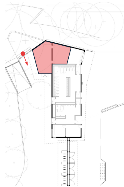
Enlarged Plan
